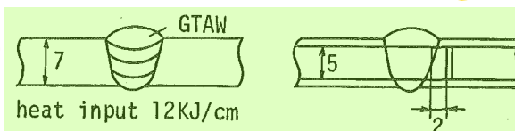
Fig.1 Welded joint for evaluation of HAZ embrittlement 11
