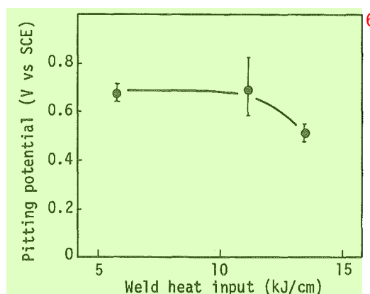
Fig.11 Effect of welding condition on pitting potential of girth weldment
