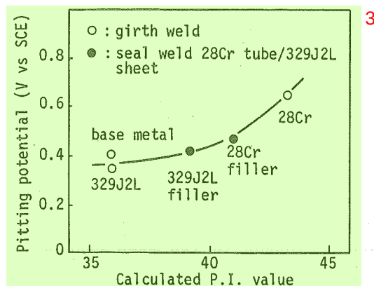
Fig.13 Pitting potential of tube-to-tube sheet weldment
