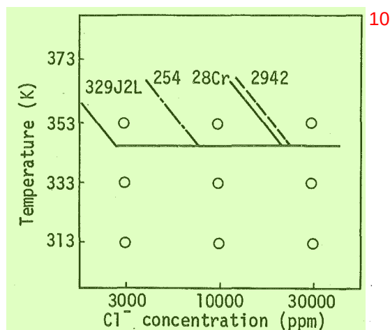
Fig. 9 Effect of temperature and chloride concentration on crevice corrosion resistance at 0.4V for 48h 10
