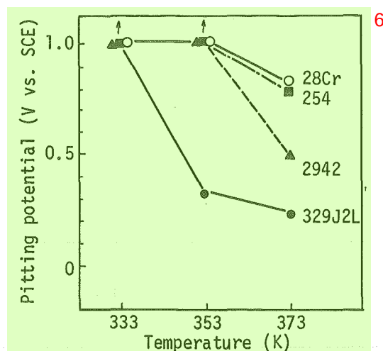
Fig. 7 Effect of temperature on pitting potential in synthetic seawater 7
