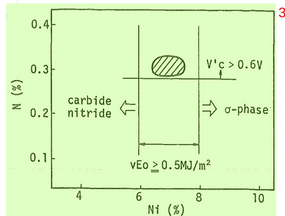
Fig.5 Optimum Ni and N content range determined by HAZ performance
