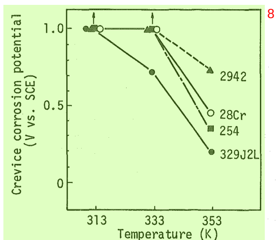
Fig. 8 Effect of temperature on crevice corrosion potential in synthetic seawater 8
