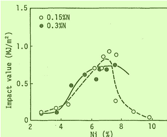
Fig.3 Effect of Ni and N content on HAZ toughness at 273K 15
