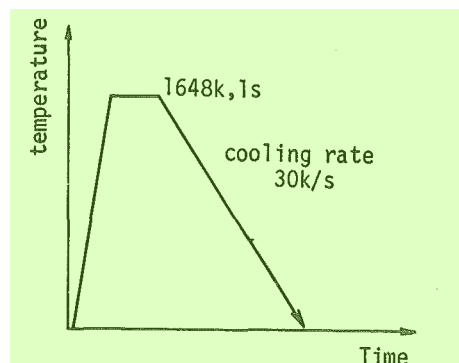
Fig.2 Thermal cycle applied to simulated HAZ specimen 13
